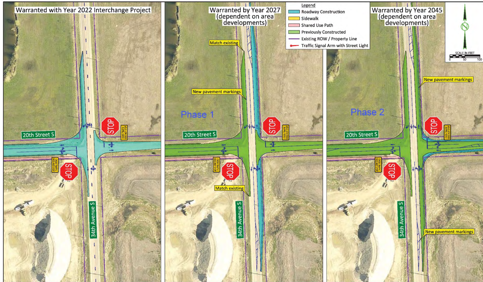
Figure 2-3. Proposed Improvements to the Intersection of 20th Street South and 34th Avenue South
