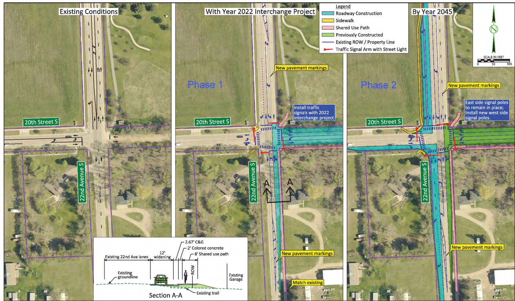
Figure 2-2. Proposed Improvements to the Intersection of 20th Street South and 22nd Avenue South
