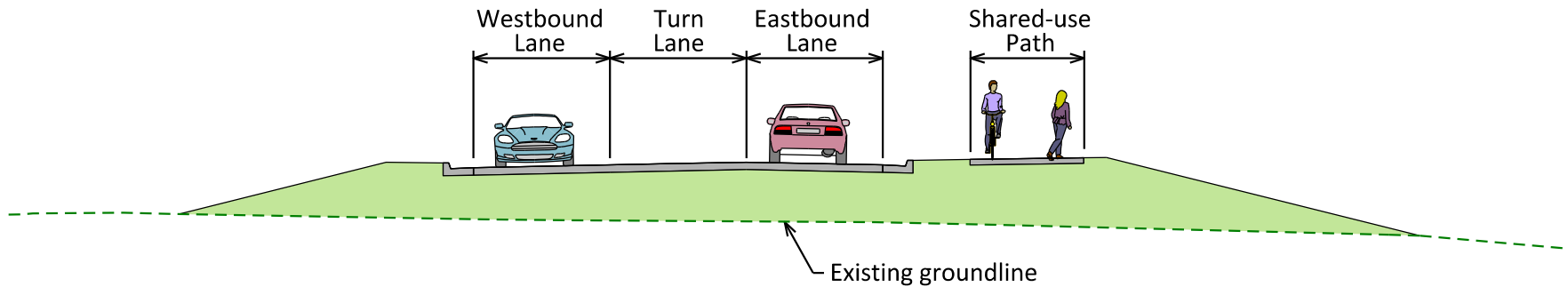
Typical 20th Street S. Section - Looking East
